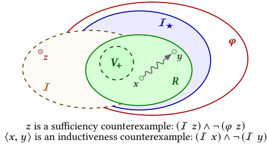
Figure 2. A sufficient representation invariant I_* implies the spec and is an overapproximation of the set of representations R of the module’s abstract type.
