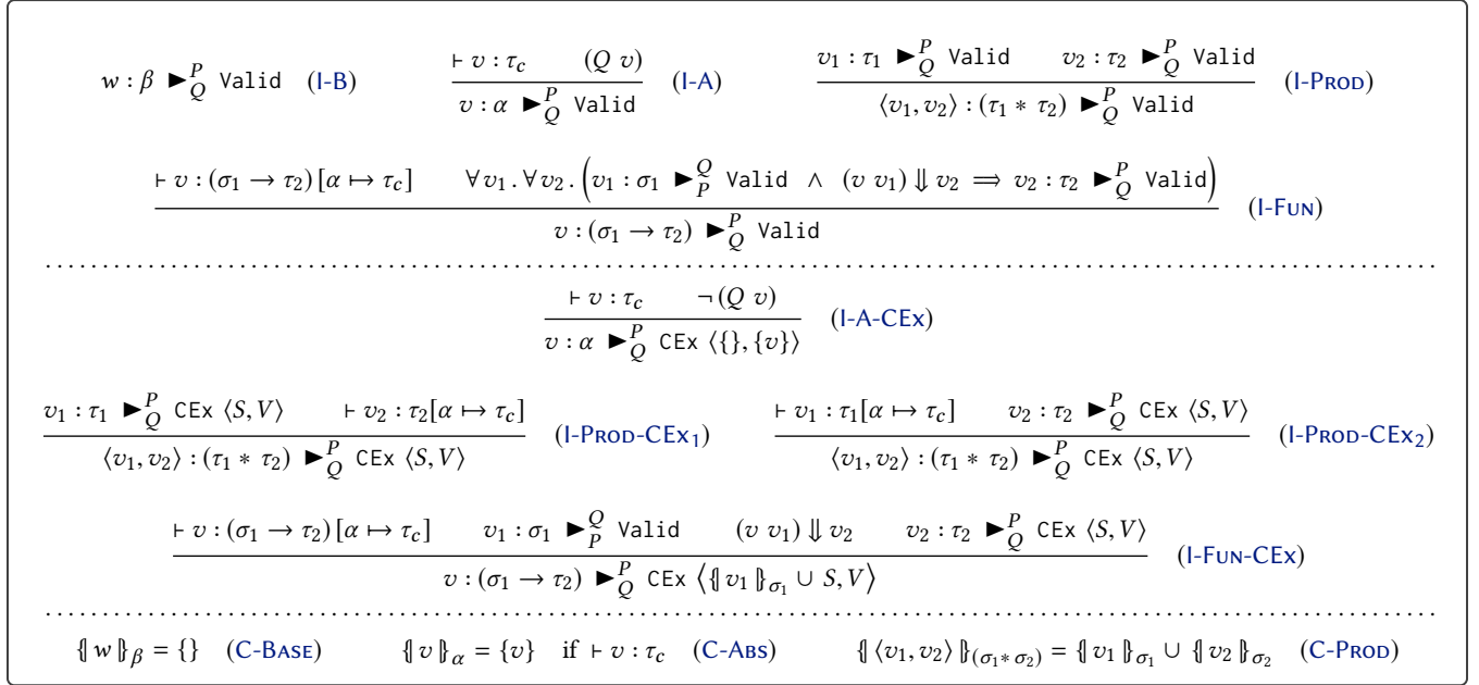
Figure 3. Inference rules for conditional inductiveness.
