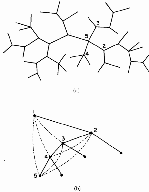
Fig. 4. A case of nonplanarity.
